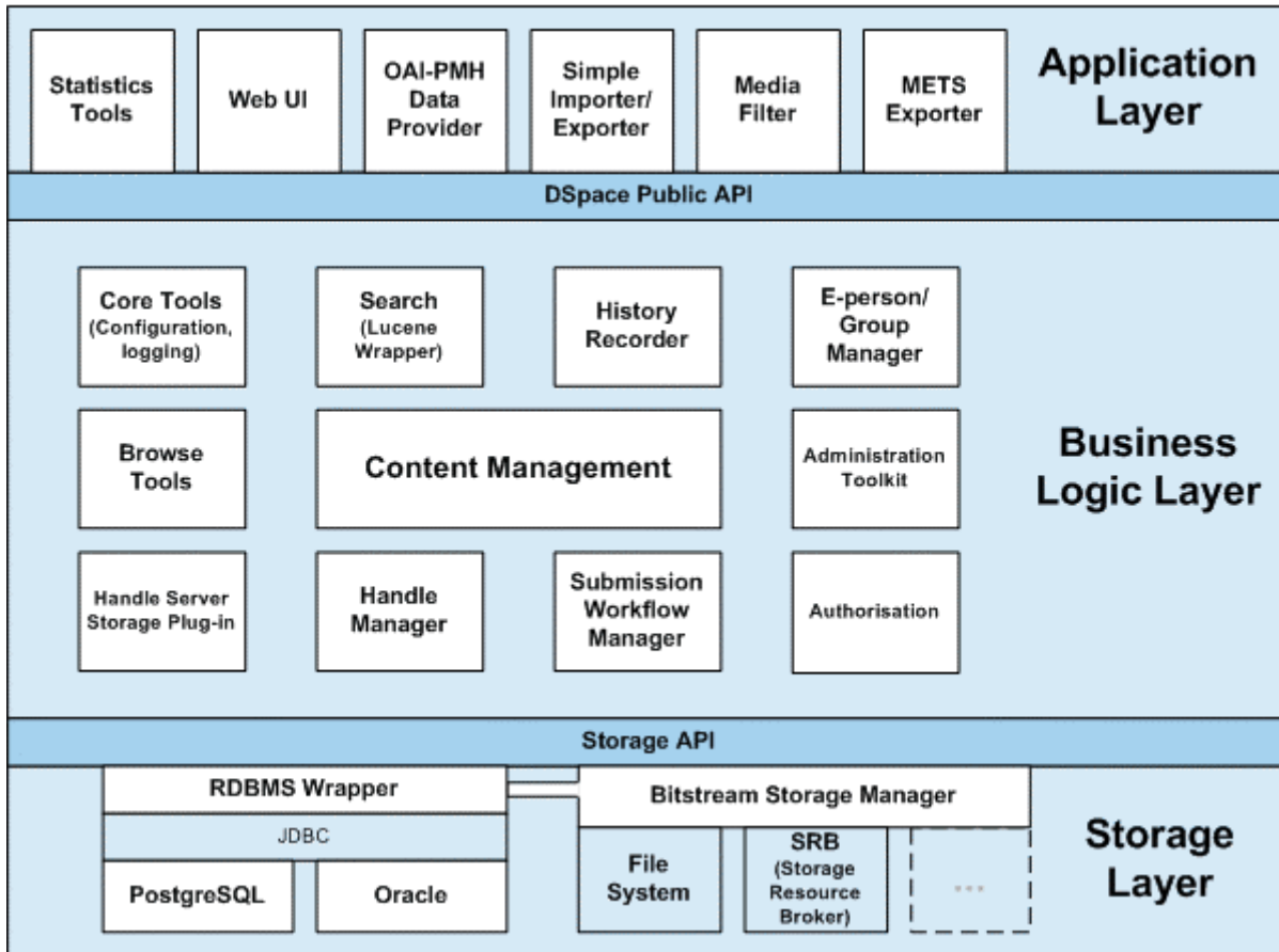
DSpace System Architecture
